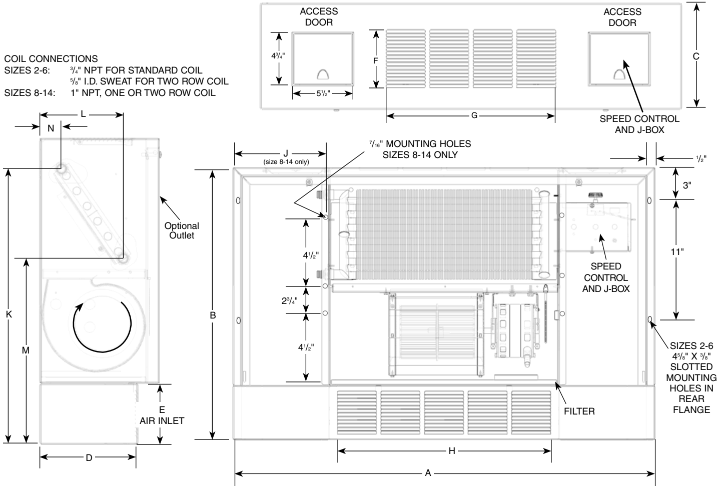
Cabinet Dimensions (inches)
