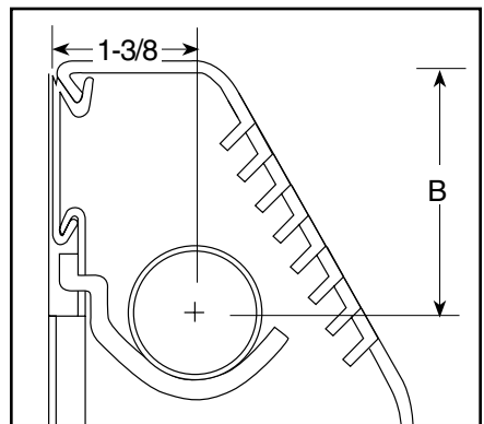
RETURN PIPE HANGER
